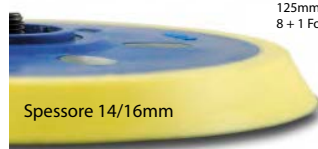
17010 125mm, 16mm Soft 8 + 1 Fori
